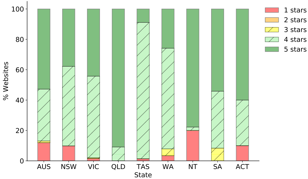
Figure 10: Rating (stars) for government websites of different states/territories based on 2020 results. AUS-fed. indicates the Australian federal government results.
