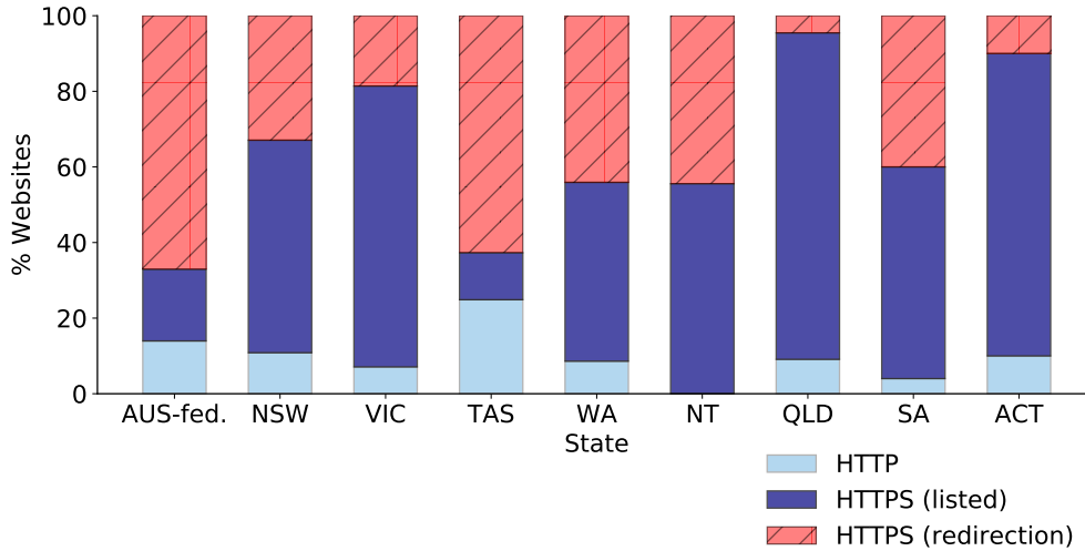
Figure 5: HTTP/HTTPS ratios for government websites of different states/territories. AUS-fed. indicates the Australian federal government.
