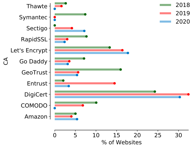
Figure 6: Top-10 Certificate Authorities (CAs) used by Australian federal government websites between 2018 and 2020.
