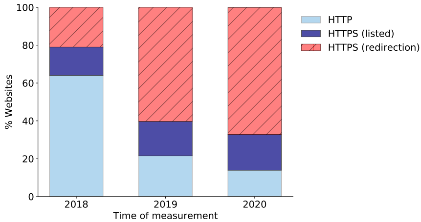
Figure 3: The use of HTTP and HTTPS protocol by Australian federal government websites. Between 2018 and 2020, the fraction of HTTPS websites has increased from 36% to 86%.
