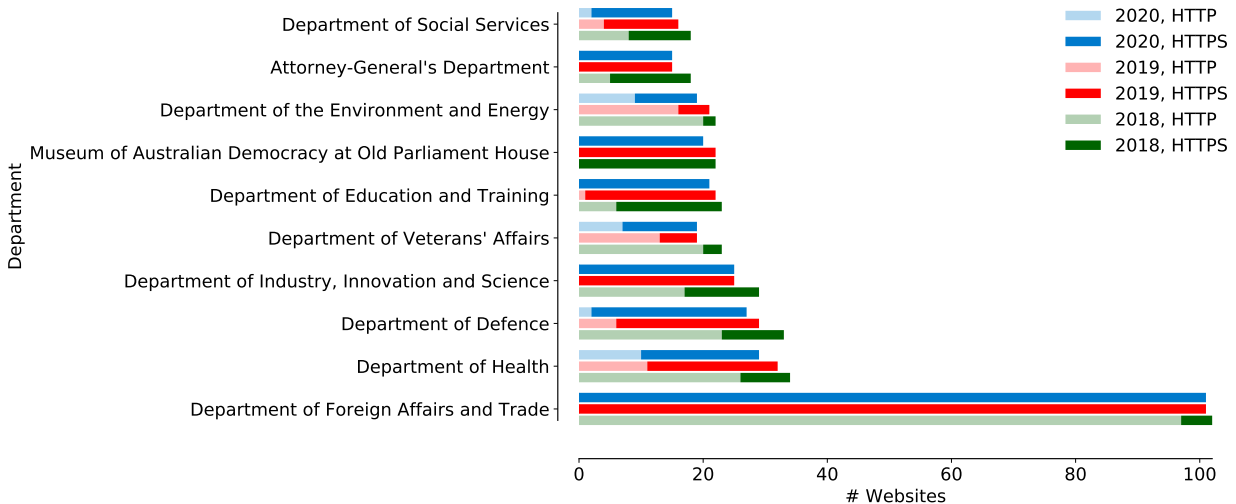
Figure 4: HTTP/HTTPS ratios for the 10 government departments with the highest number of listed websites.
