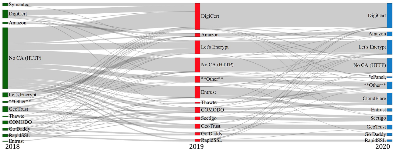
Figure 7: Certificate Authority (CA) transitions of Australian federal government websites from 2018 to 2020.
