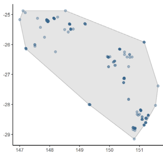
Figure 2. Construction of minimum convex polygon for Extent of Occurrence ( Eucalyptus panda )
